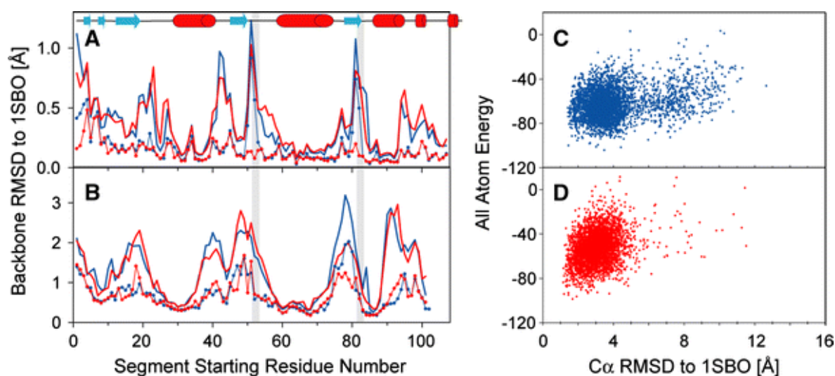
Fig. 4 CS-Rosetta structure generation of TM1442 with chemical shift errors. A, B Plots of accuracy of fragments selected using the MFR ( blue ) and hybrid ( red ) methods, with the inputs swapped for the \delta^{15}\text{N} , \delta^1\text{H}^{\text{N}} , \delta^{13}\text{C}^{\alpha} , \delta^{13}\text{C}^{\beta} , \delta^{13}\text{C}' and \delta^1\text{H}^{\alpha} assignments of dipeptides Ser 52 -Ser 53 and Ser 82 -Ser 83 (as contained in the dataset IIIb ). For each 3-residue ( A ) and 9-residue ( B ) segment of TM1442, 200 fragments were selected. Average ( bold lines ) and lowest ( lines with dots ) rmsd of these fragments relative to the experimental coordinates of the corresponding TM1442 segment are plotted with respect to the position of the first segment residue in the TM1442 sequence. The regions corresponding to the “miss-assigned” residues are shaded; secondary structure elements are displayed at the top. C, D Plots of Rosetta all atom energy, rescored by using the input chemical shifts (as contained in the dataset IIIb ), versus C \alpha rmsd relative to the experimental TM1442 structure, for CS-Rosetta models obtained using MFR ( C ) and hybrid ( D ) fragment selection methods
