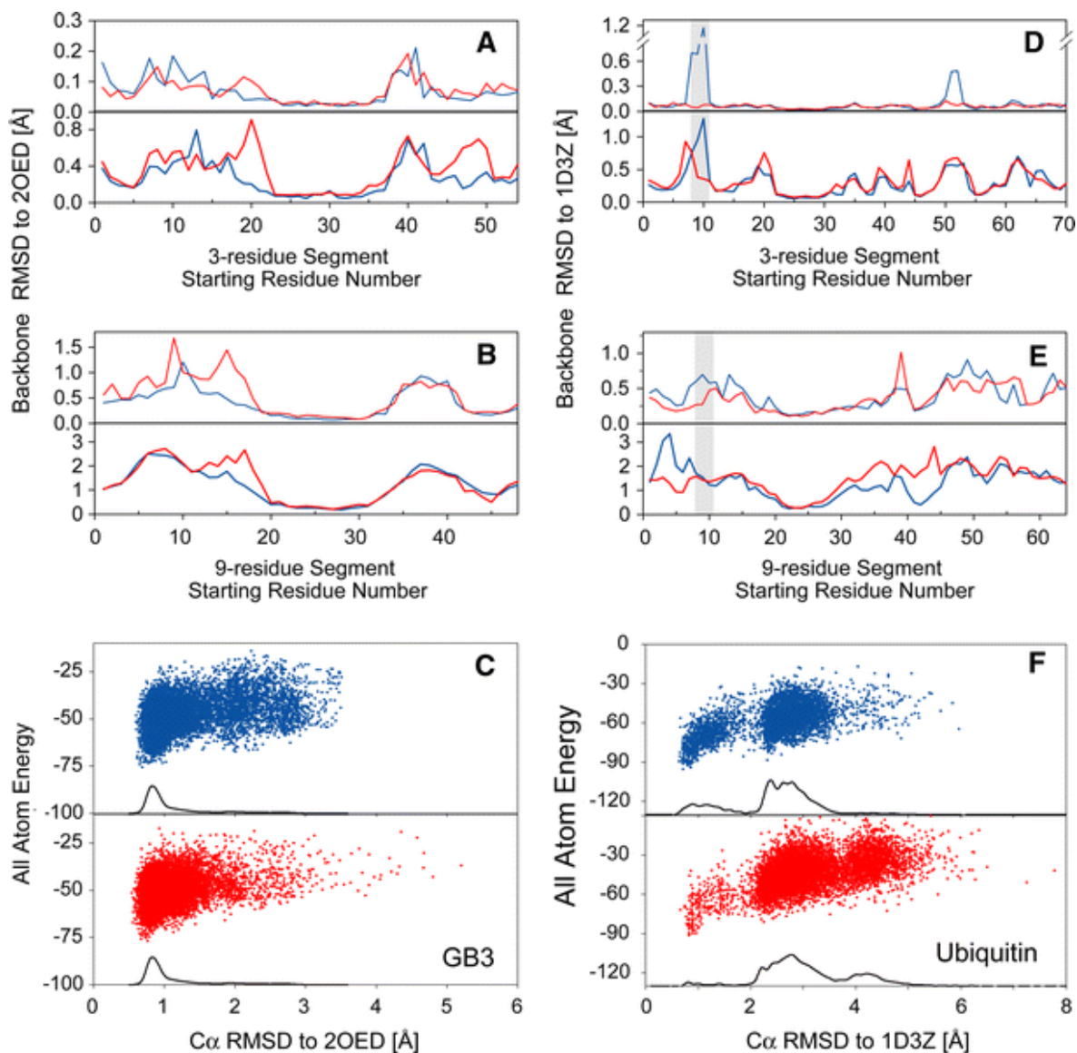
Fig. 5 CS-Rosetta fragment selection and structure generation for GB3 ( A–C ) and ubiquitin ( D–F ), using chemical shift assignments from solid-state NMR. A, D Plots of the lowest (upper panel) and average (lower panel) backbone coordinate rmsds (N, C α and C') between query segment and two hundred 3-residue fragments, selected using the MFR ( blue ) and hybrid methods ( red ), as a function of starting position in the sequence. B, E Same as ( A, D ), but for 9-residue fragments. C, F Plots of Rosetta all atom energy, rescored by using the experimental ssNMR chemical shifts, versus C α rmsd relative to the experimental NMR structures of GB3 and ubiquitin for the CS-Rosetta all-atom models obtain using MFR-selected (upper panel, blue dots ) and the hybrid method (lower panel, red dots ) fragments. The solid black lines in ( C, F ) represent the normalized number of structures found at a given C α -rmsd
