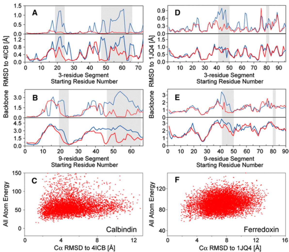
Fig. 6 CS-Rosetta structure generation for paramagnetic calbindin ( A–C ) and ferredoxin ( D–F ). A, D Plots of the lowest (upper panel) and average (lower panel) backbone coordinate rmsds (N, C ^{\alpha} and C') between query segment and two hundred 3-residue fragment candidates, selected using the MFR ( blue ) and hybrid methods ( red ), as a function of starting position in the sequence. The regions lacking chemical shift assignments are shaded. B, E Same as ( A, D ), but for 9-residue fragments. C, F Plots of Rosetta all-atom energy, rescored by the experimental chemical shifts, versus C ^{\alpha} rmsd of final all-atom models (including only residues located in elements of secondary structure) relative to the corresponding X-ray (calbindin) and NMR (ferredoxin) structure. Only results from CS-Rosetta all-atom models obtained by the hybrid fragment selection procedure are shown; when using fragments from the standard MFR method, Rosetta fails to converge. Residues included in the backbone rmsd calculation include 3–14, 25–40, 46–53 and 63–74 for calbindin, and 4–11, 15–22, 27–34, 54–56, 71–75 and 91–93 for ferredoxin
