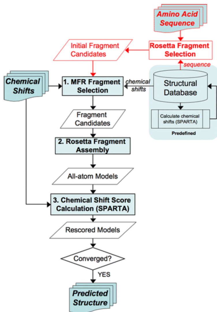
Fig. 1 Flow chart of CS-Rosetta structure generation protocol. In the hybrid fragment selection procedure, shown in red, step 1 selects 200 fragments from an initial cohort of 2,000 fragments which has been extracted from the structural database by standard Rosetta methods. In the standard CS-Rosetta method, step 1 takes its fragments directly from the 2,200,000 fragments present in the structural database
