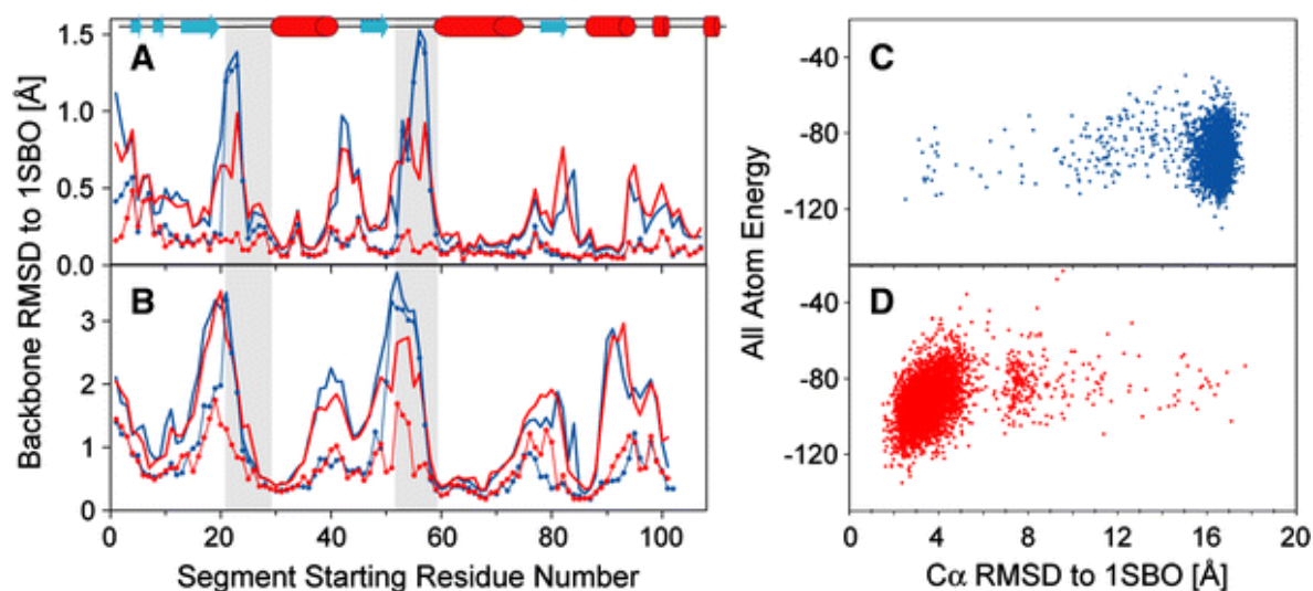
Fig. 3 CS-Rosetta structure for TM1442 with missing chemical shifts. A, B Plots of accuracy of fragment candidates selected using the MFR ( blue ) and hybrid ( red ) methods using chemical shift values \delta^{15}\text{N} , \delta^1\text{H}^{\text{N}} , \delta^{13}\text{C}^{\alpha} , \delta^{13}\text{C}^{\beta} , \delta^{13}\text{C}^{\gamma} and \delta^1\text{H}^{\alpha} for residues 1–20, 30–51 and 60–120 (as contained in the dataset Ie ). For each 3-residue ( A ) and 9-residue ( B ) segment of TM1442, 200 fragments were selected. Average ( bold lines ) and lowest ( lines with dots ) rmsd of these fragments relative to the experimental coordinates of the corresponding TM1442 segment are plotted with respect to the position of the first segment residue in the TM1442 sequence. The regions corresponding to the “unassigned” residues are shaded; the secondary structure elements are displayed at the top. C, D Plots of Rosetta all atom energy, rescored by using the input chemical shifts (as contained in dataset Ie ), versus \text{C}^{\alpha} rmsd relative to the experimental TM1442 structure, for CS-Rosetta models obtained using MFR ( C ) and hybrid ( D ) fragment selection methods
