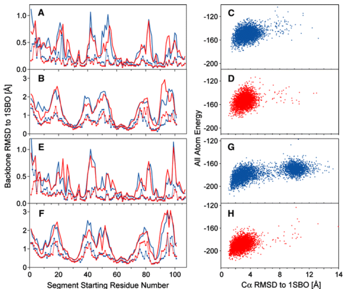
Fig. 2 CS-Rosetta structure generation for TM1442 with missing chemical shift assignments for certain types of nuclei. A, B Plots of accuracy of fragments selected using the MFR ( blue ) and hybrid ( red ) methods with the chemical shift inputs for \delta^{15}\text{N} , \delta^1\text{H}^\text{N} and \delta^{13}\text{C}^\alpha (as contained in dataset lh ). Quality of 3-residue ( A ) and 9-residue ( B ) fragments is represented by the average ( bold lines ) and lowest ( lines with dots ) rmsd of 200 selected fragments relative to the
