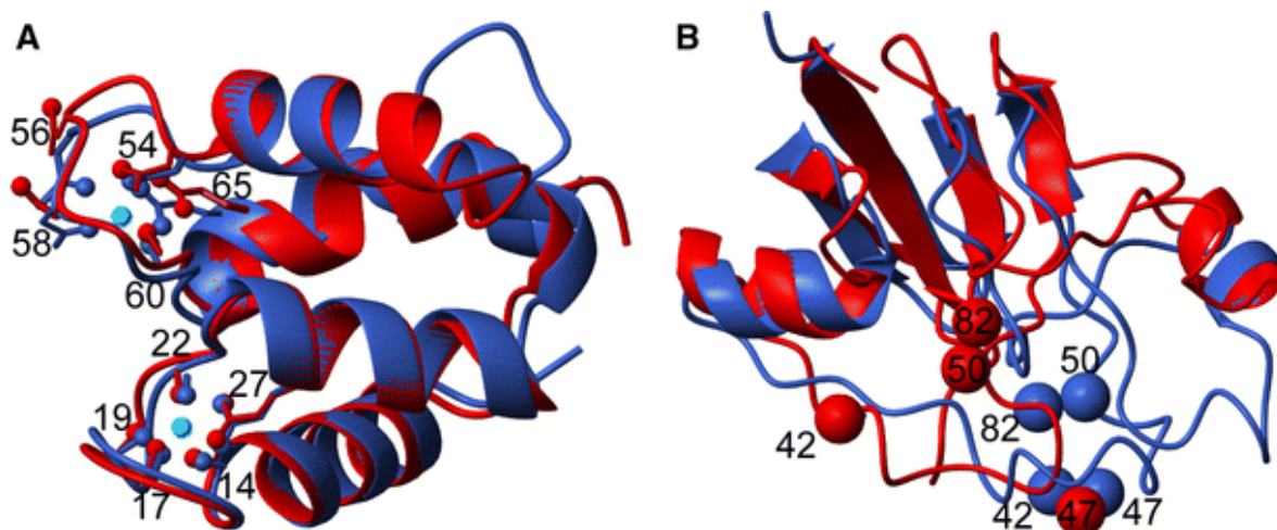
Fig. 7 Comparison of experimental ( blue ) and lowest energy CS-Rosetta ( red ) structure for paramagnetic calbindin ( A )
