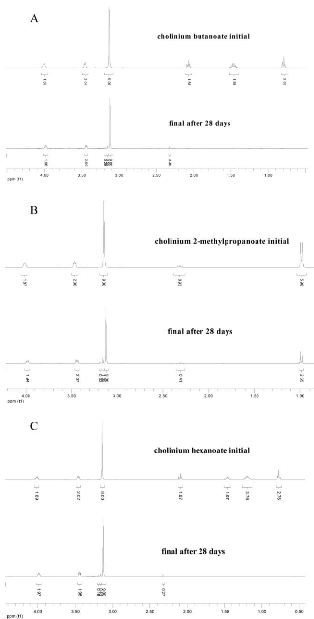
Fig. 5 Biodegradability assessment using Penicillium corylophilum . ^1\text{H} NMR spectra at the beginning and the end of the incubation period (28 days) for (A) cholinium butanoate (0.1 M), (B) cholinium 2-methylpropanoate (0.1 M), and (C) cholinium hexanoate (0.05 M).
