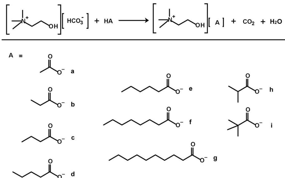
Fig. 1 Chemical route for obtaining the cholinium alkanooate ionic liquids, [NMe 3 (CH 2 CH 2 OH)][C n H 2n+1 CO 2 ] (n = 1-9) and chemical structures of the anions used: (a) ethanoate, (b) propanoate, (c) butanoate, (d) pentanoate, (e) hexanoate, (f) octanoate, (g) decanoate, (h) 2-methylpropanoate, (i) 2,2-dimethylpropanoate.
